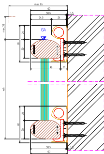
GM WINDOORAIL® profiel ovaal
